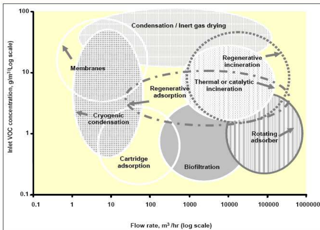
Figure 20.5: Overview of application ranges of the available VOC abatement technologies [60, ESIG, 2000]
