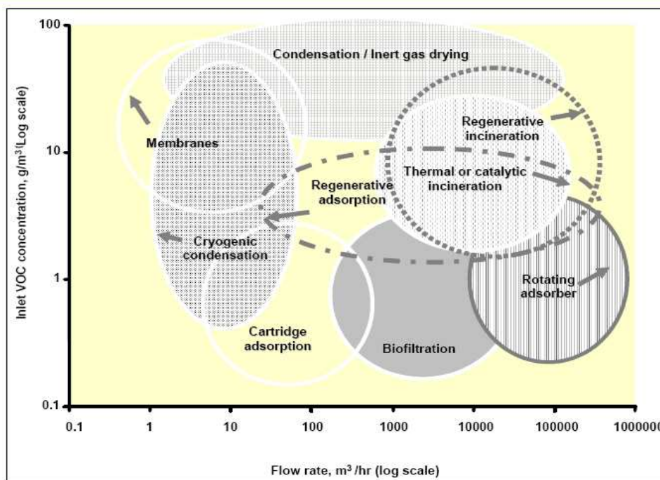
Figure 20.5: Overview of application ranges of the available VOC abatement technologies [60, ESIG, 2000]
