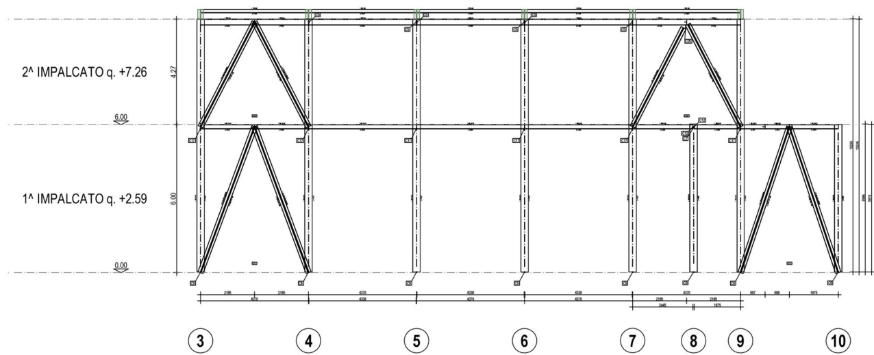
Telaio 3-4-5-6-7-8-9-10
