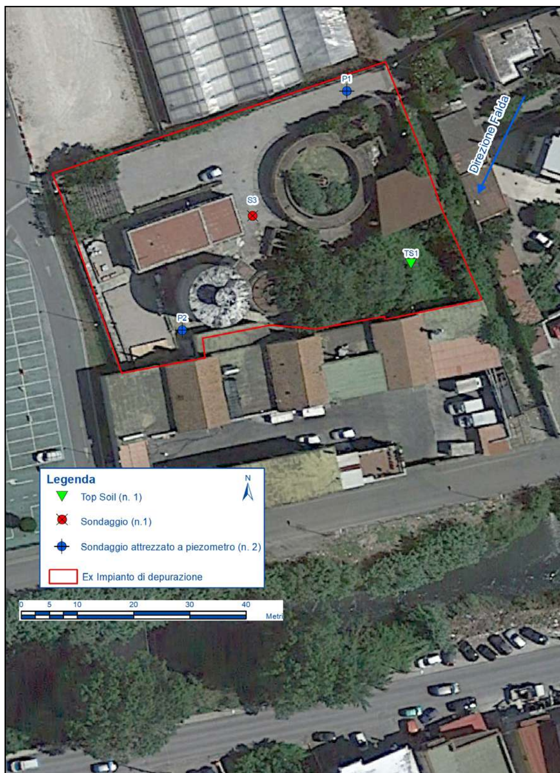
Figura 5 – Piano d’Indagine
